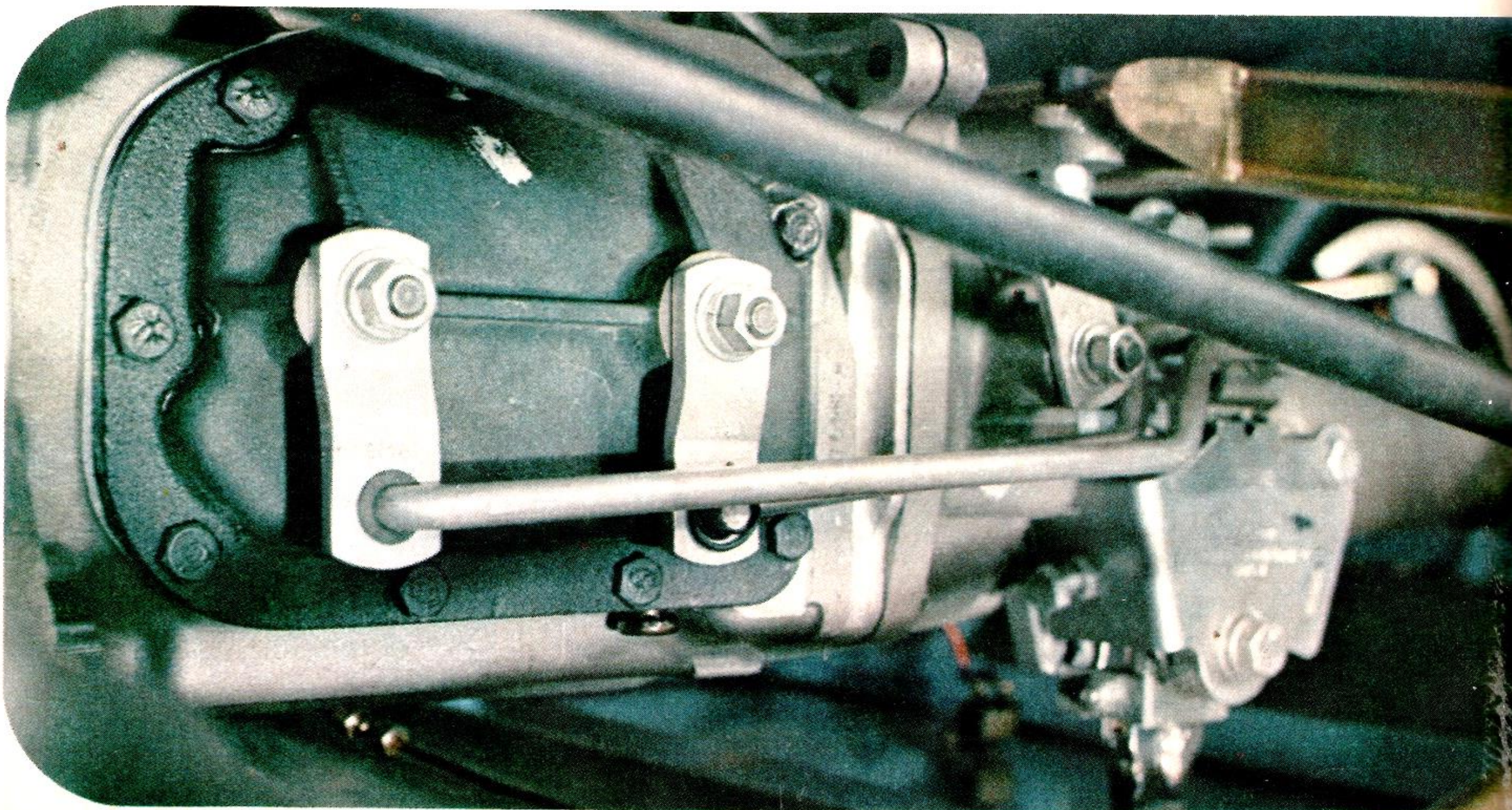
Many transmissions will be called upon during initial phase of program to determine best one possible for 1683-pound car. Choices consist of experimental 2-speed auto, B-W T-10, Ford four-speed.
