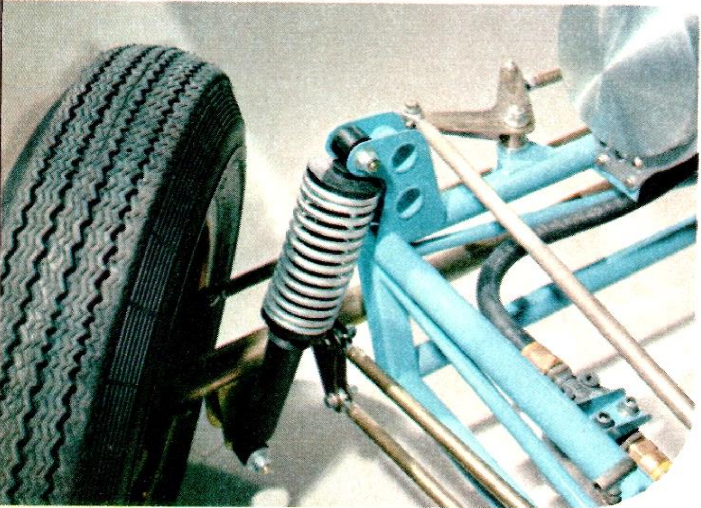
At top we note method of locating "Daytona" type rear end assembly by 1 1/4-inch square tube composed traction truss. Long, curved calipers are Mustang-breed with beefed castings. Suspension is Autolite coil/shocks both front and rear.
