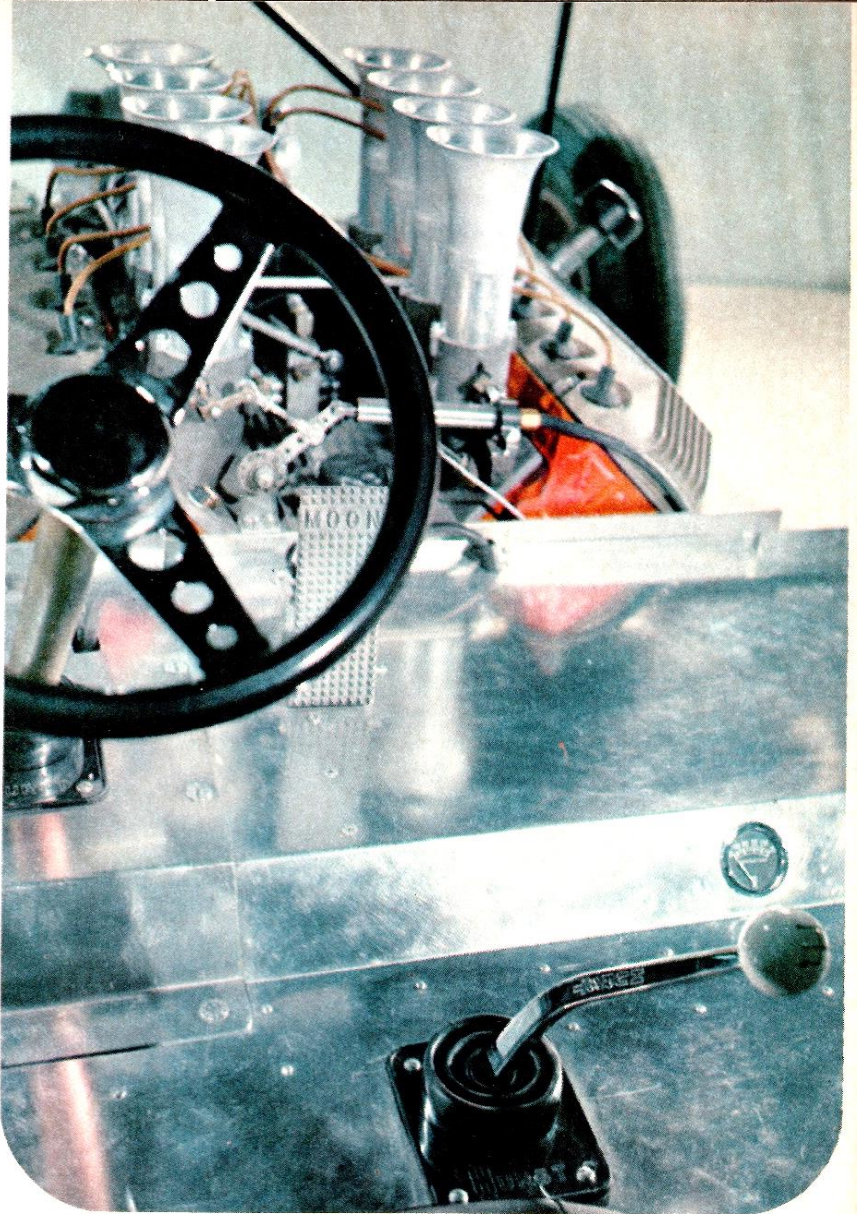
RIGHT — Pale reflection in the .030-inch aluminum floor backdrops bold Covico steering wheel, forest of Hilborn tubes. Dead-sure shifts by Hurst.
